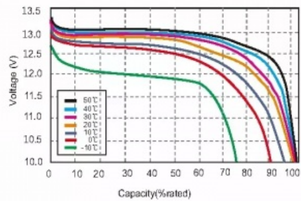
Different Temperature Discharge Curve @0.5C
