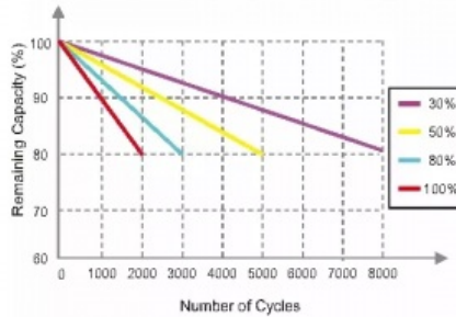
Different DOD Discharge Cycle Life Curve @1C
