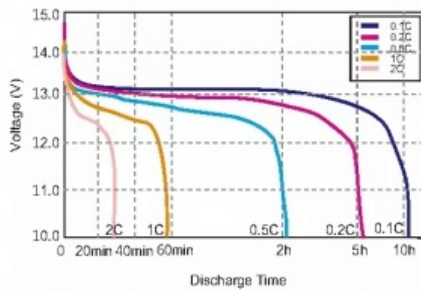
Different Rate Discharge Curve @25°C
