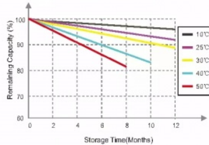
Different Temperature Self Discharge Curve
