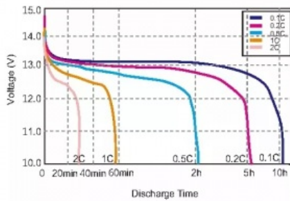
Different Rate Discharge Curve @25°C
