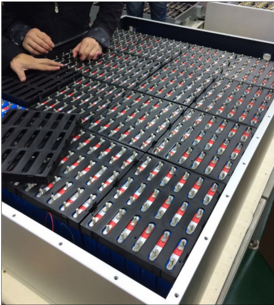
Producing Line
